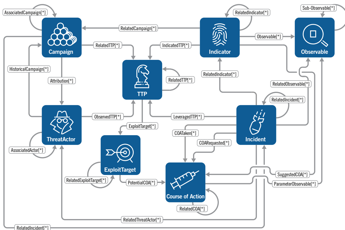
Figure 1. Diagram of the STIX taxonomy ( https://stixproject.github.io/about/ )
